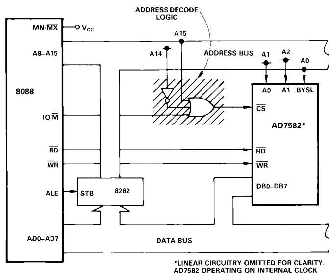
Figure 21. AD7582 – 8088 Interface
